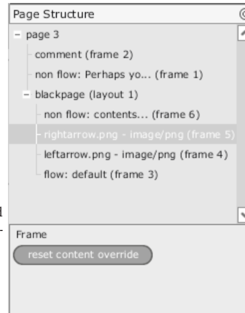
The page structure palette with a frame on the template selected.
